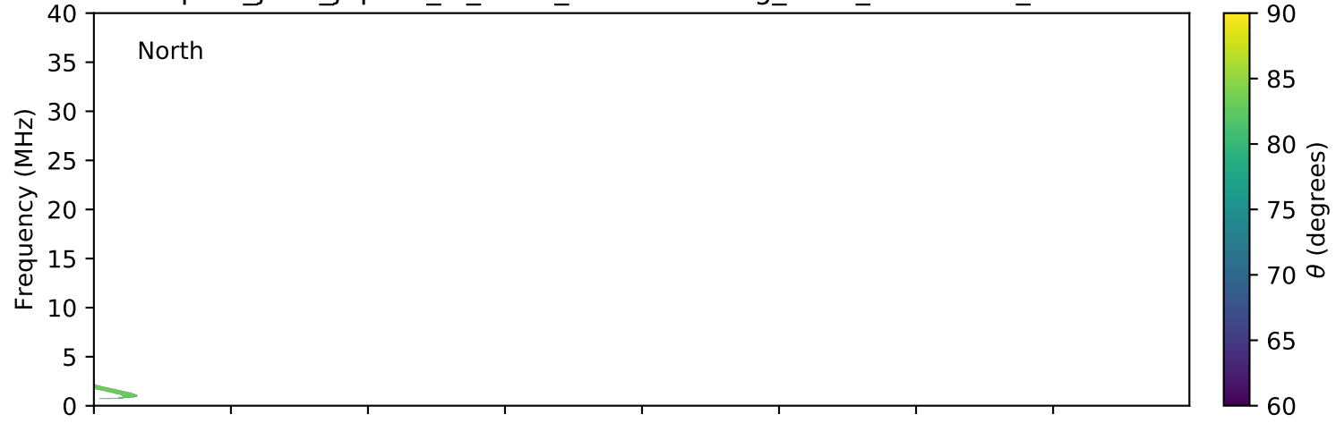
expres_juno_jupiter_io_isaac_lossc-wid1deg_3kev_20170918_v01.cdf
