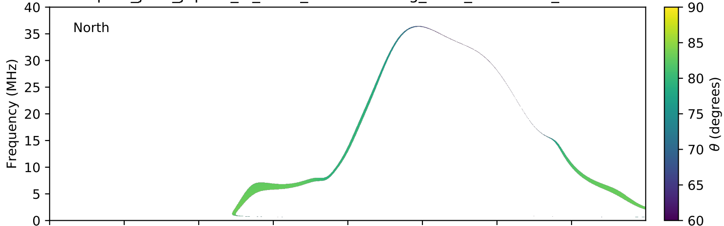
expres_juno_jupiter_io_isaac_lossc-wid1deg_3kev_20170917_v01.cdf
