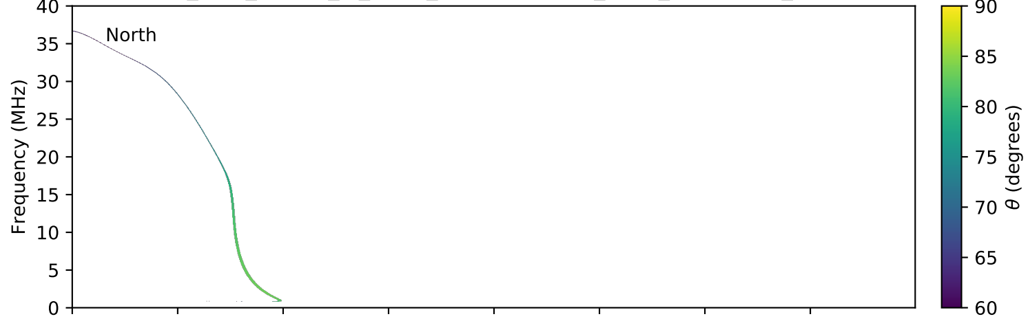
expres_juno_jupiter_io_isaac_lossc-wid1deg_3kev_20170916_v01.cdf
