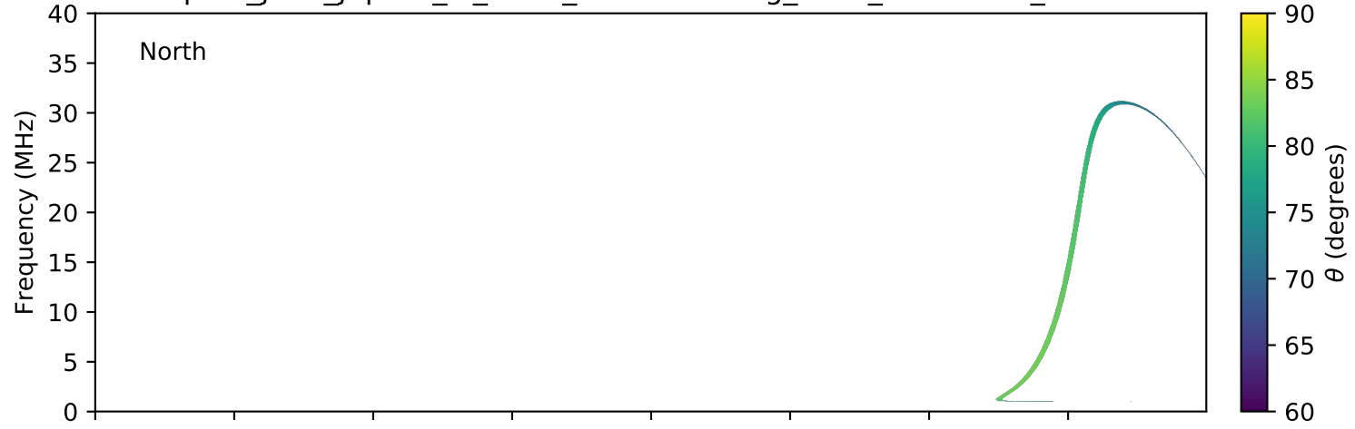
expres_juno_jupiter_io_isaac_lossc-wid1deg_3kev_20170913_v01.cdf
