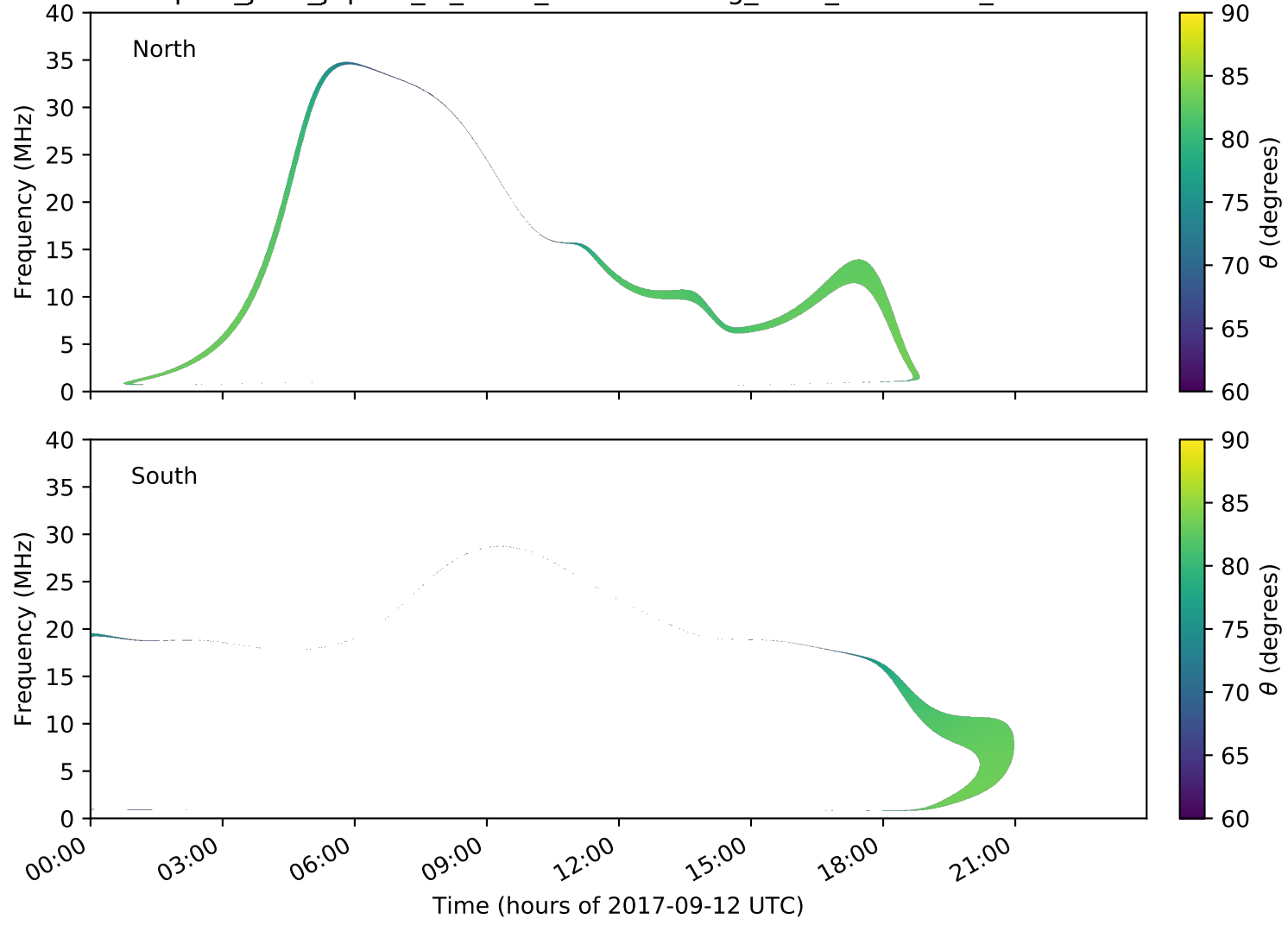
expres_juno_jupiter_io_isaac_lossc-wid1deg_3kev_20170912_v01.cdf
