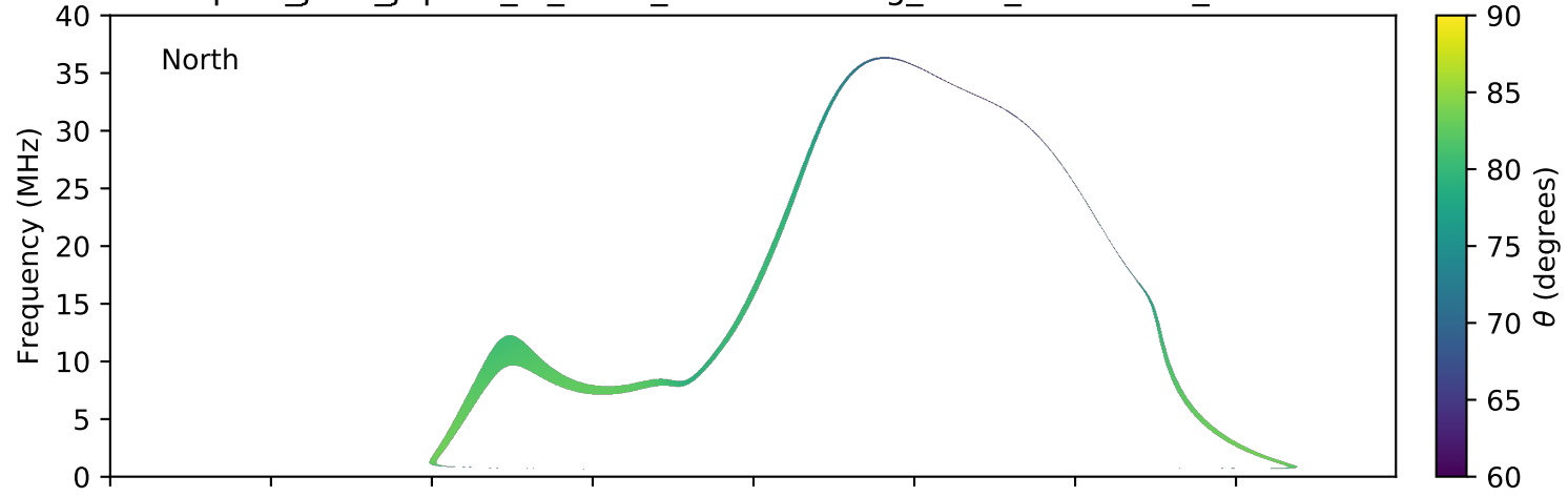
expres_juno_jupiter_io_isaac_lossc-wid1deg_3kev_20170910_v01.cdf
