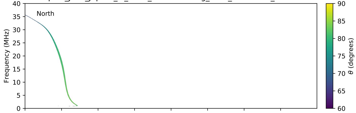
expres_juno_jupiter_io_isaac_lossc-wid1deg_3kev_20170909_v01.cdf
