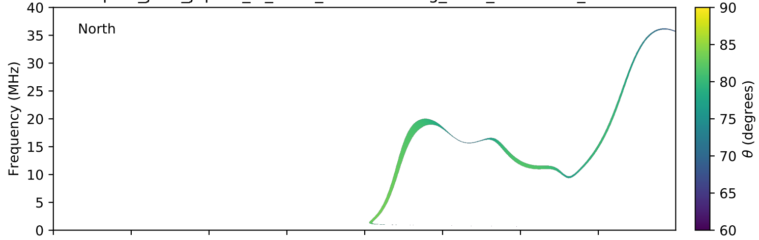
expres_juno_jupiter_io_isaac_lossc-wid1deg_3kev_20170908_v01.cdf
