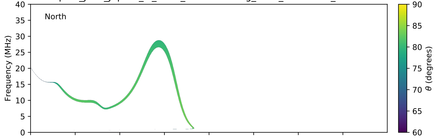
expres_juno_jupiter_io_isaac_lossc-wid1deg_3kev_20170907_v01.cdf
