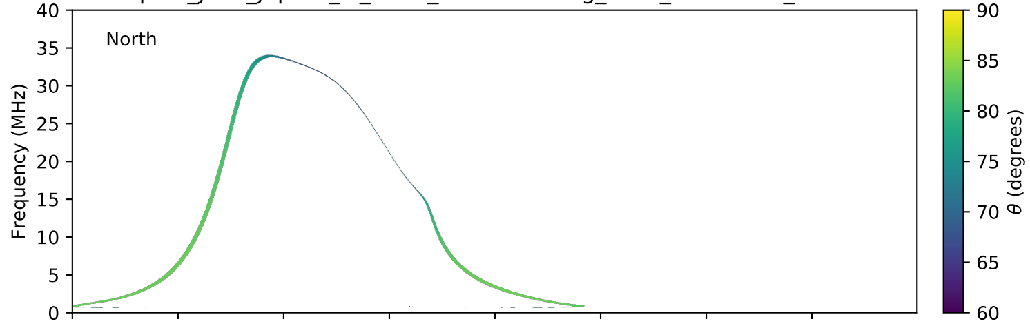
expres_juno_jupiter_io_isaac_lossc-wid1deg_3kev_20170905_v01.cdf
