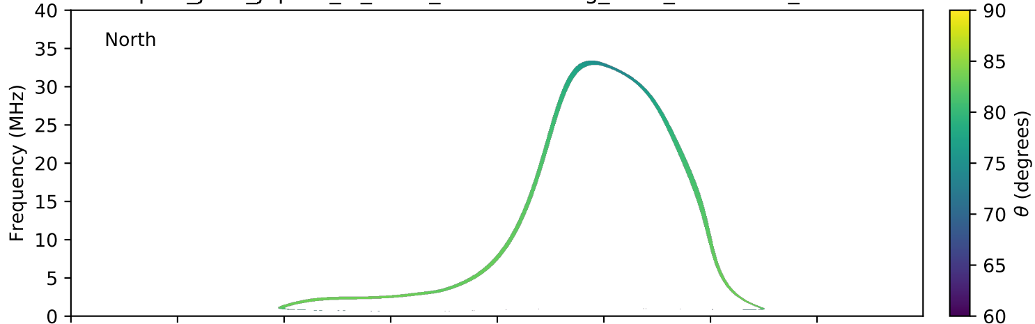
expres_juno_jupiter_io_isaac_lossc-wid1deg_3kev_20170903_v01.cdf
