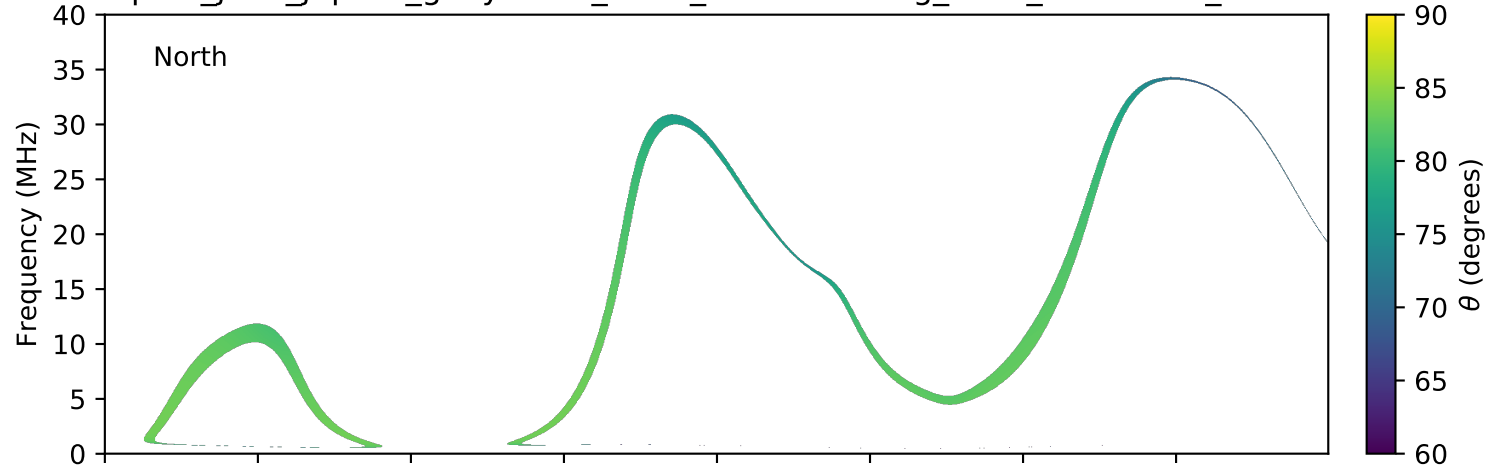
expres_juno_jupiter_ganymede_isaac_lossc-wid1deg_3kev_20170930_v01.cdf
