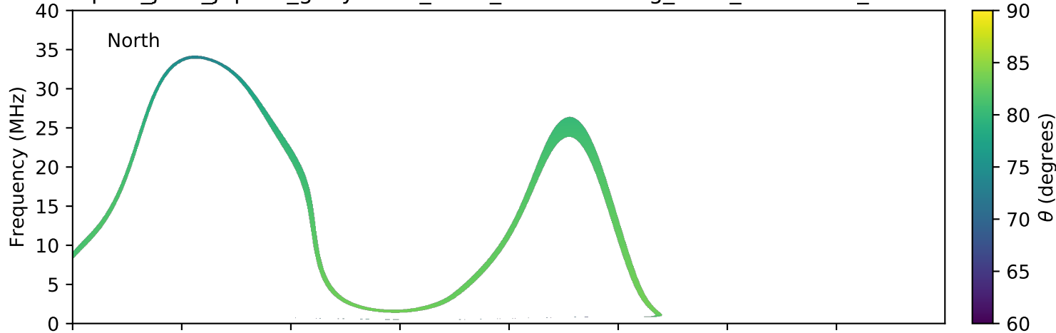
expres_juno_jupiter_ganymede_isaac_lossc-wid1deg_3kev_20170925_v01.cdf
