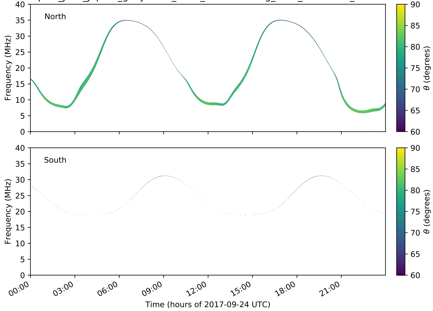
expres_juno_jupiter_ganymede_isaac_lossc-wid1deg_3kev_20170924_v01.cdf
