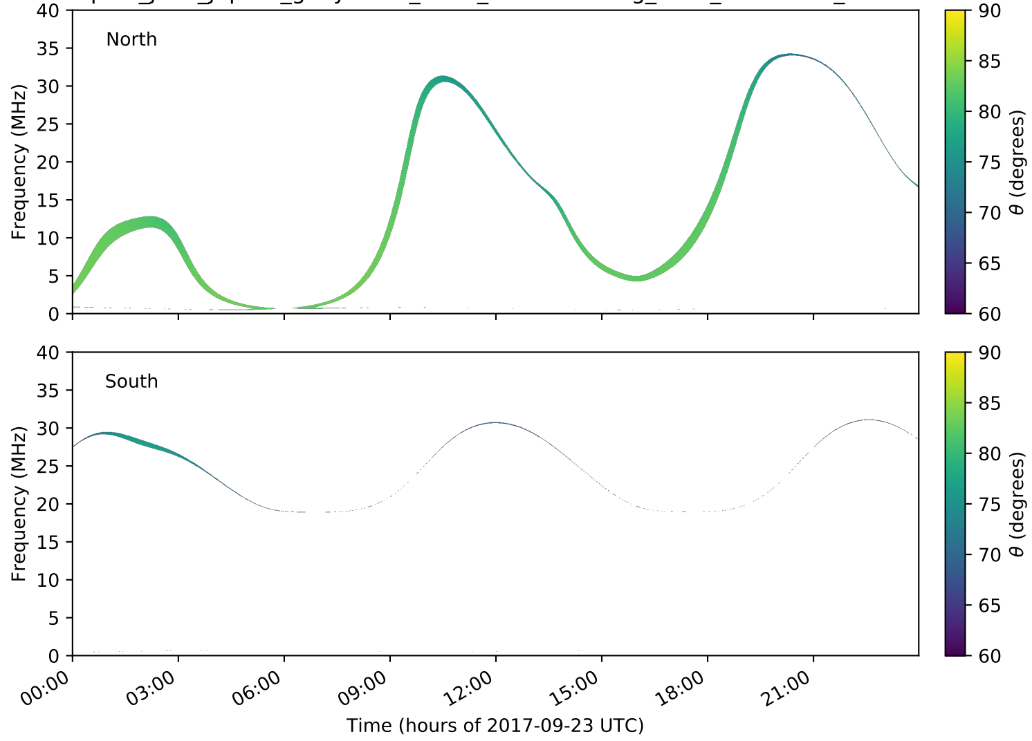
expres_juno_jupiter_ganymede_isaac_lossc-wid1deg_3kev_20170923_v01.cdf
