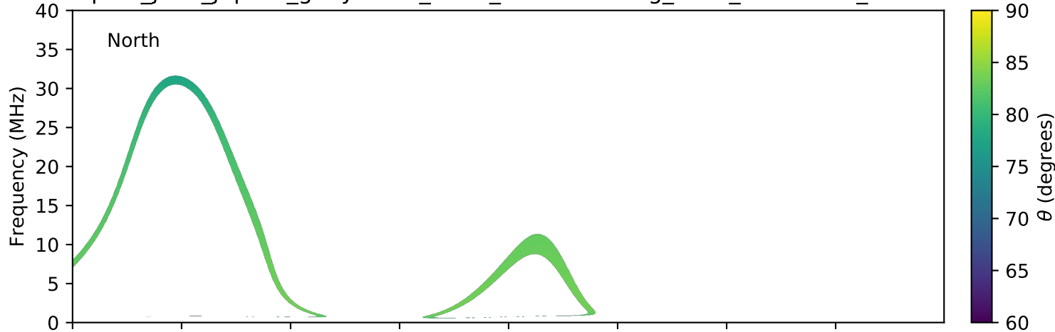
expres_juno_jupiter_ganymede_isaac_lossc-wid1deg_3kev_20170918_v01.cdf
