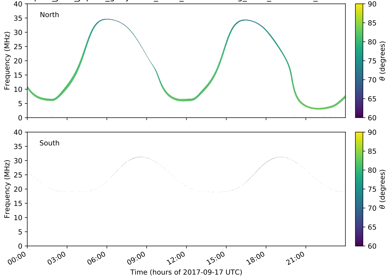
expres_juno_jupiter_ganymede_isaac_lossc-wid1deg_3kev_20170917_v01.cdf
