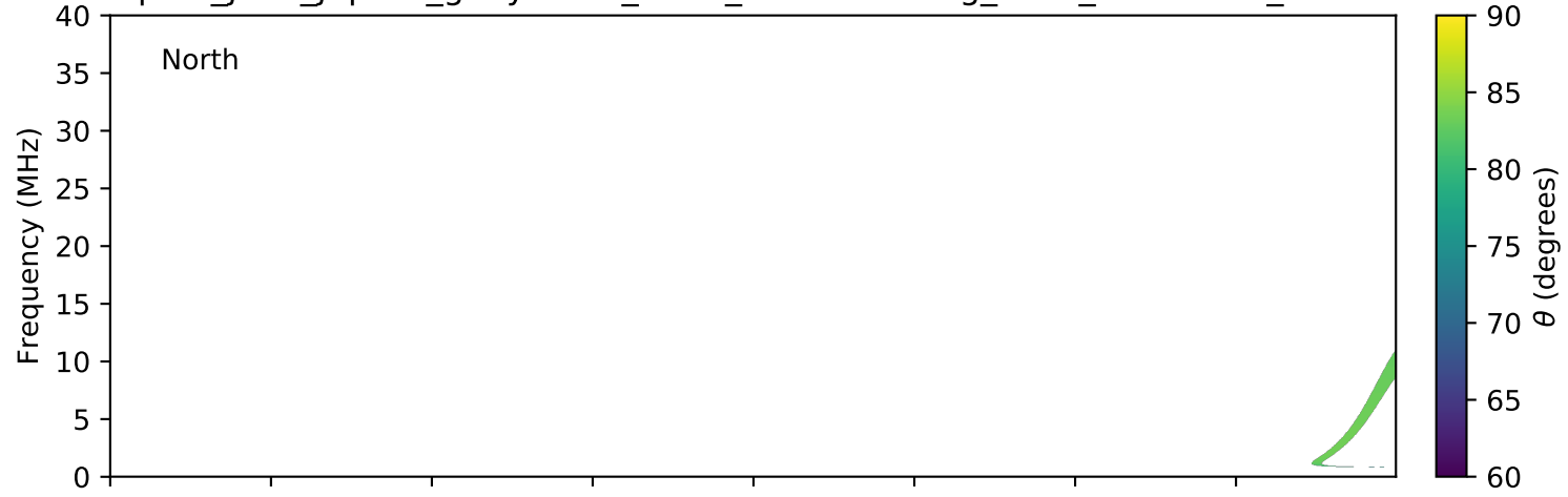
expres_juno_jupiter_ganymede_isaac_lossc-wid1deg_3kev_20170915_v01.cdf
