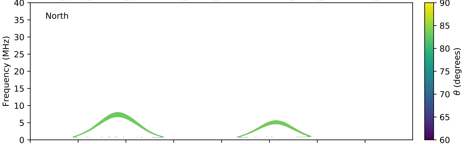
expres_juno_jupiter_ganymede_isaac_lossc-wid1deg_3kev_20170903_v01.cdf
