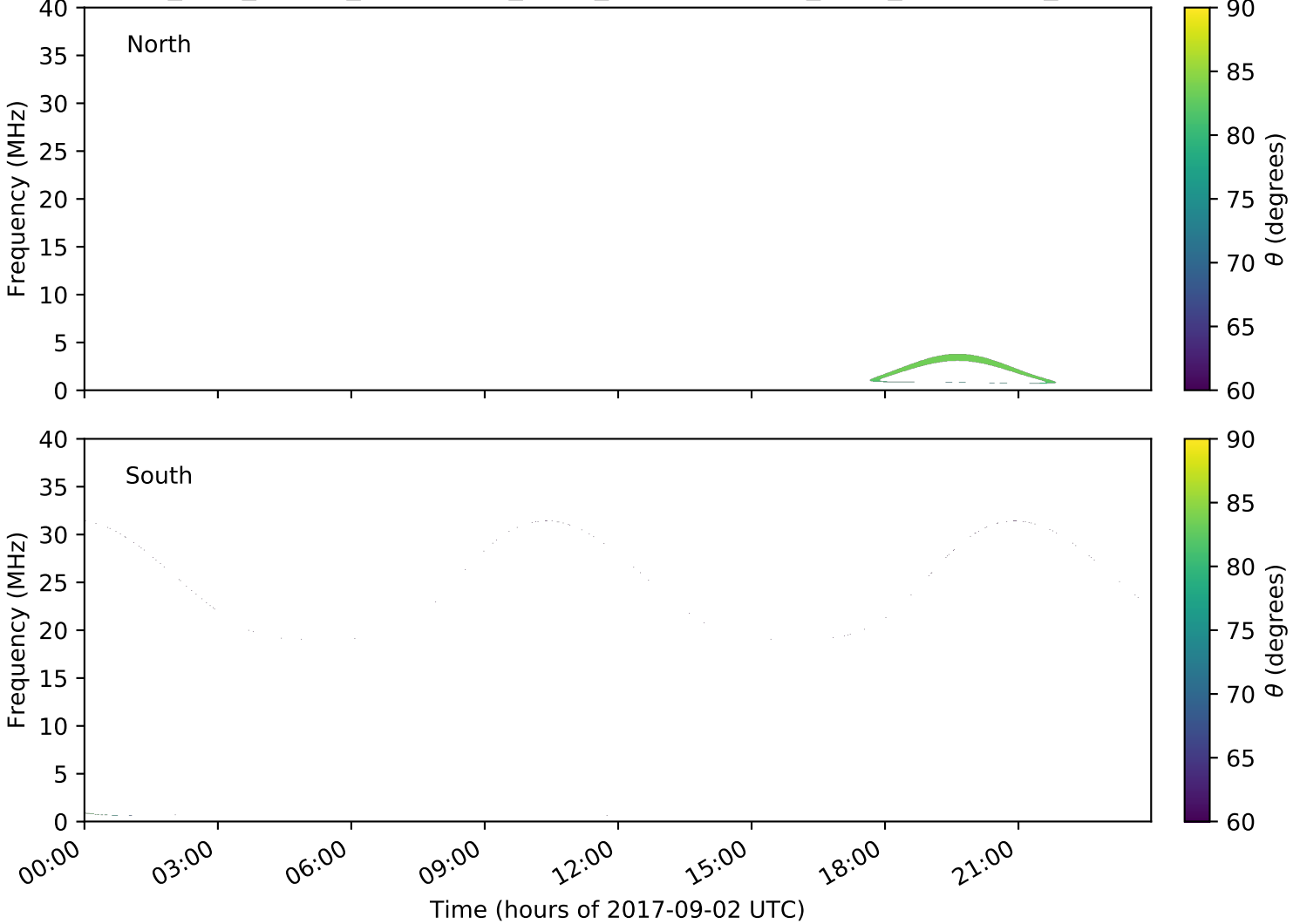
expres_juno_jupiter_ganymede_isaac_lossc-wid1deg_3kev_20170902_v01.cdf
