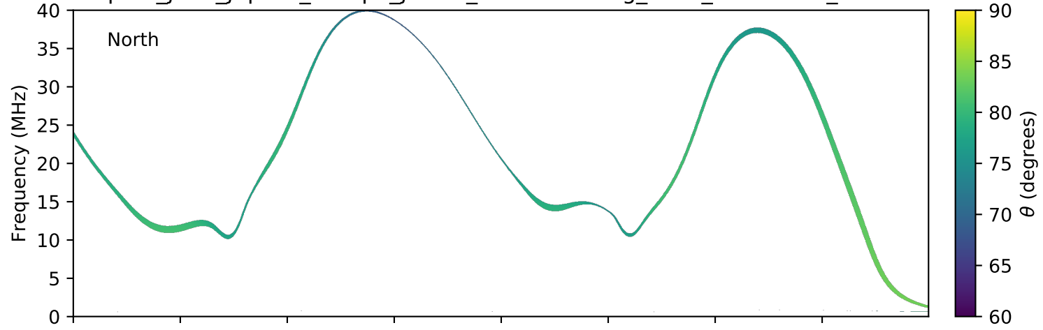
expres_juno_jupiter_europa_jrm09_lossc-wid1deg_3kev_20170926_v01.cdf
