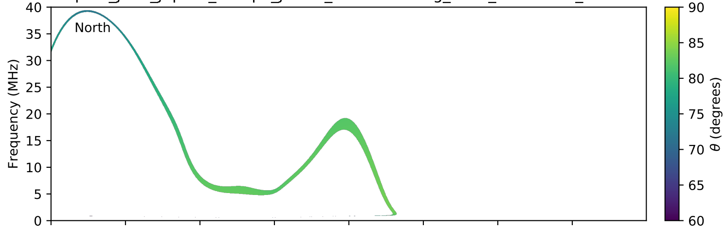
expres_juno_jupiter_europa_jrm09_lossc-wid1deg_3kev_20170923_v01.cdf
