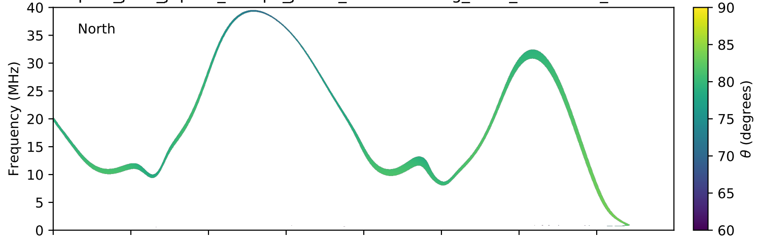
expres_juno_jupiter_europa_jrm09_lossc-wid1deg_3kev_20170919_v01.cdf
