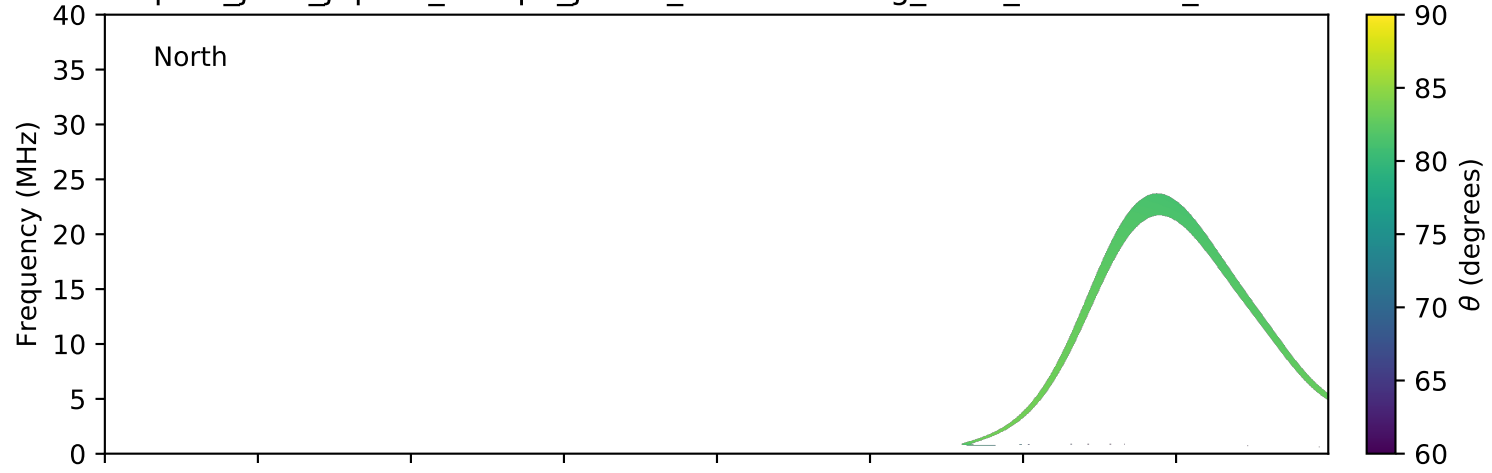
expres_juno_jupiter_europa_jrm09_lossc-wid1deg_3kev_20170904_v01.cdf
