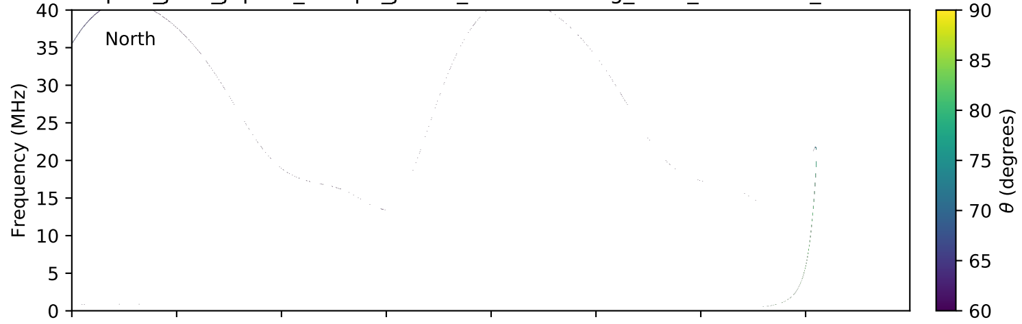
expres_juno_jupiter_europa_jrm09_lossc-wid1deg_3kev_20170901_v01.cdf
