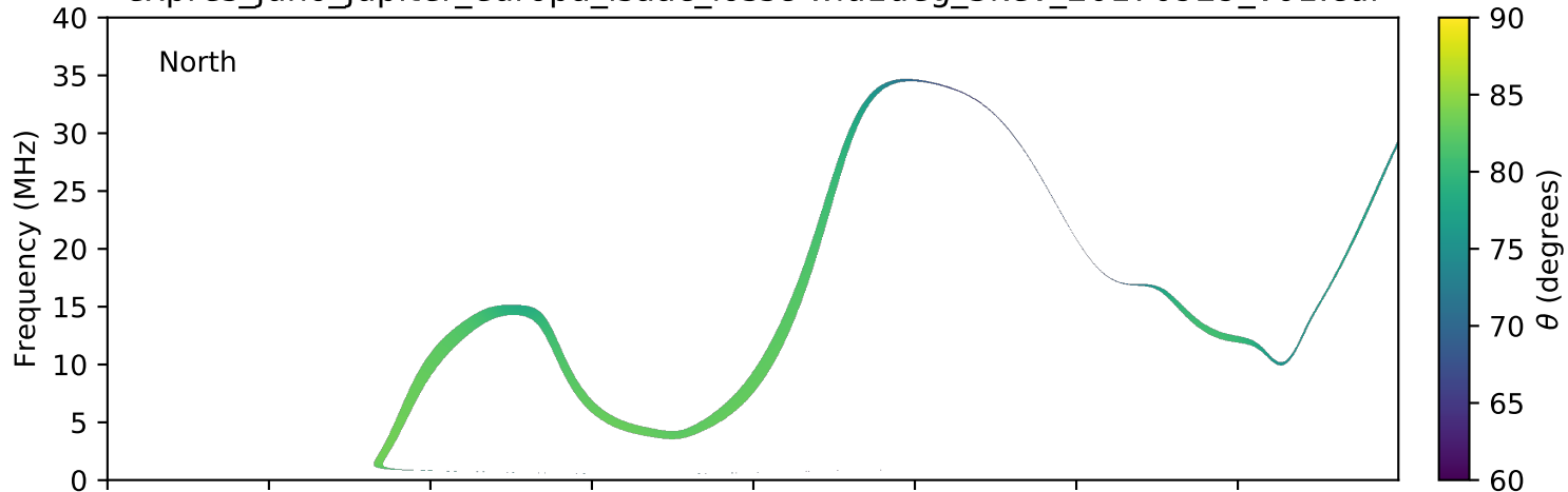
expres_juno_jupiter_europa_isaac_lossc-wid1deg_3kev_20170929_v01.cdf
