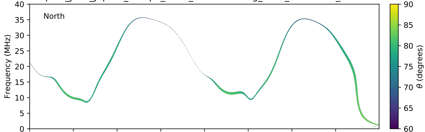
expres_juno_jupiter_europa_isaac_lossc-wid1deg_3kev_20170926_v01.cdf
