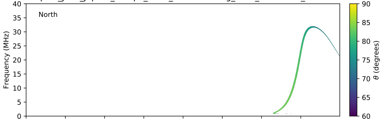
expres_juno_jupiter_europa_isaac_lossc-wid1deg_3kev_20170925_v01.cdf
