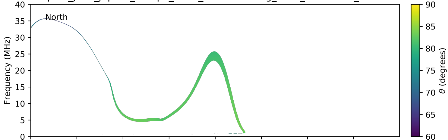
expres_juno_jupiter_europa_isaac_lossc-wid1deg_3kev_20170923_v01.cdf
