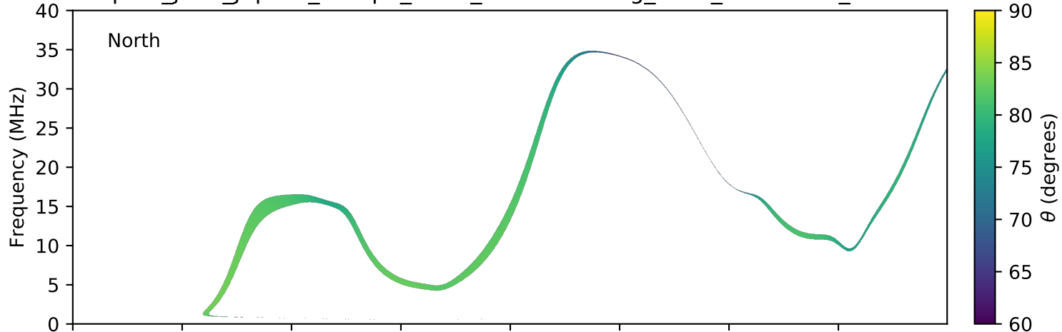
expres_juno_jupiter_europa_isaac_lossc-wid1deg_3kev_20170922_v01.cdf
