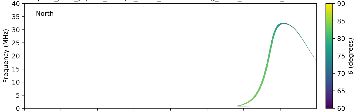
expres_juno_jupiter_europa_isaac_lossc-wid1deg_3kev_20170918_v01.cdf
