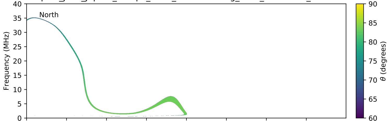
expres_juno_jupiter_europa_isaac_lossc-wid1deg_3kev_20170916_v01.cdf
