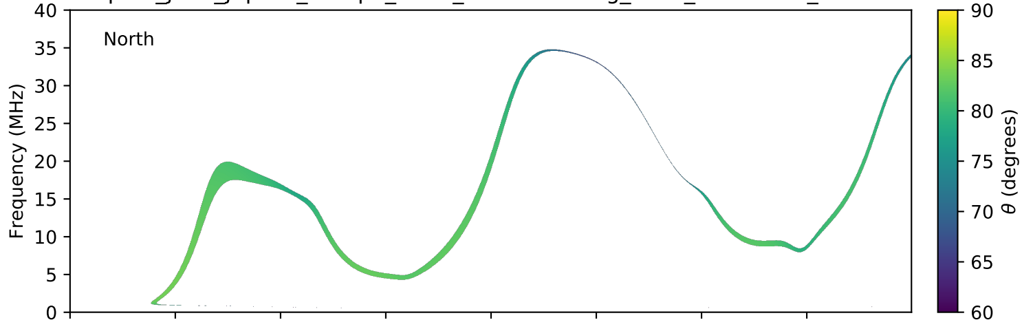
expres_juno_jupiter_europa_isaac_lossc-wid1deg_3kev_20170915_v01.cdf
