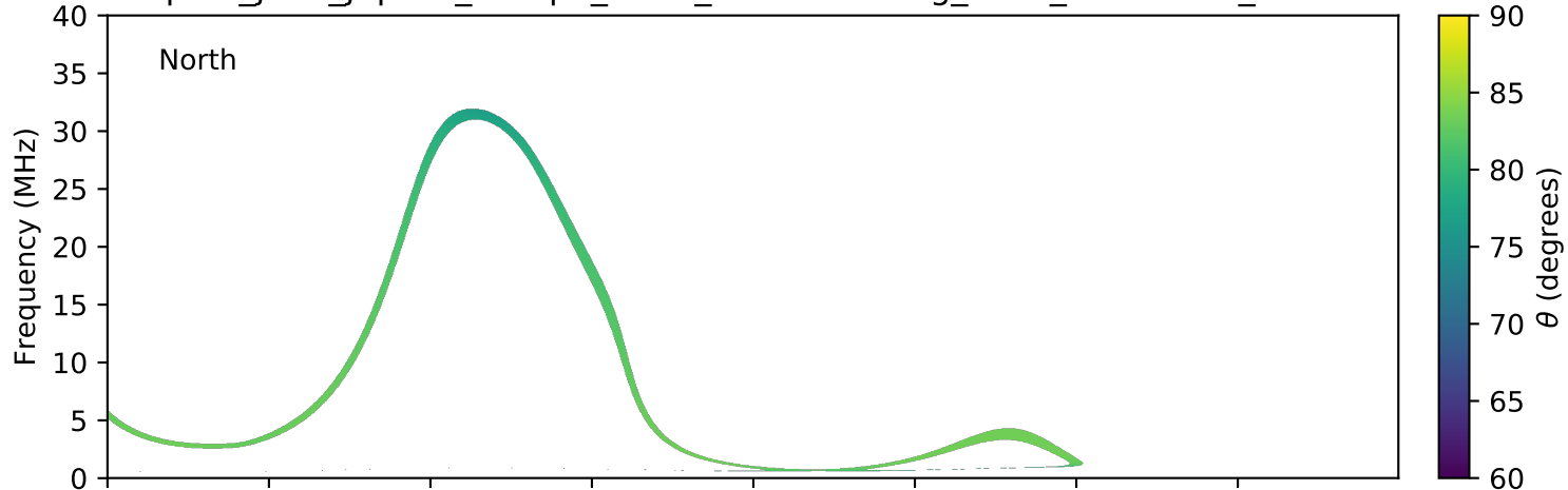
expres_juno_jupiter_europa_isaac_lossc-wid1deg_3kev_20170905_v01.cdf
