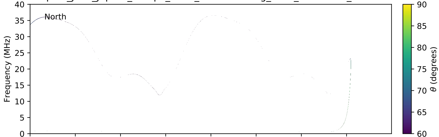
expres_juno_jupiter_europa_isaac_lossc-wid1deg_3kev_20170901_v01.cdf
