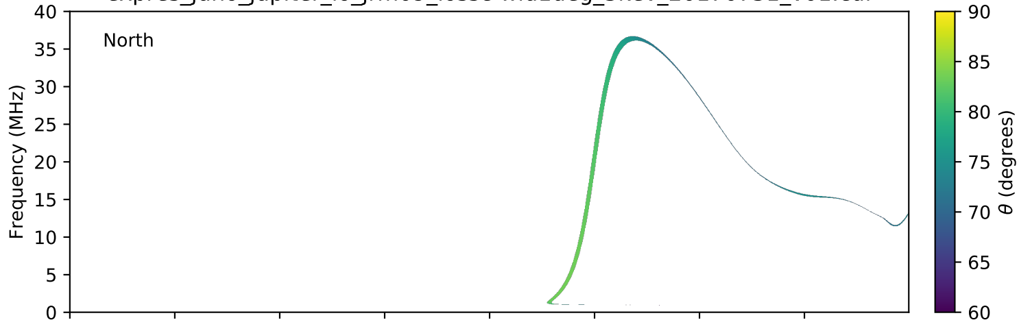
expres_juno_jupiter_io_jrm09_lossc-wid1deg_3kev_20170731_v01.cdf
