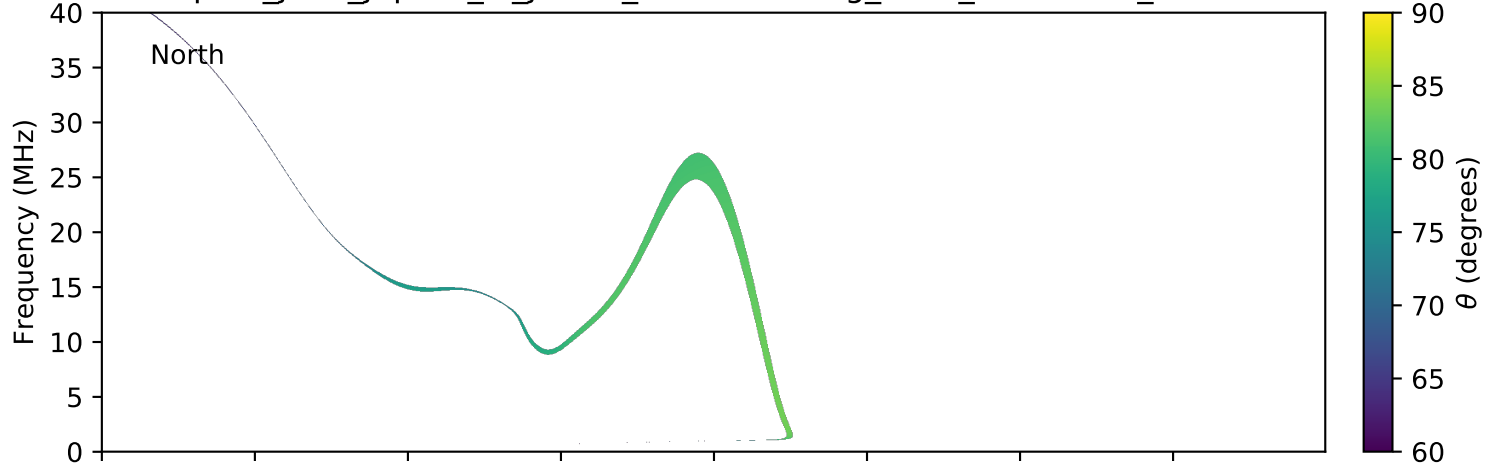
expres_juno_jupiter_io_jrm09_lossc-wid1deg_3kev_20170730_v01.cdf
