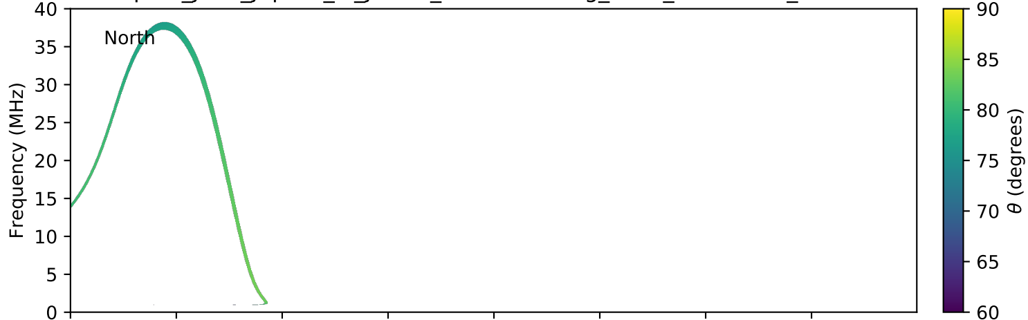
expres_juno_jupiter_io_jrm09_lossc-wid1deg_3kev_20170725_v01.cdf
