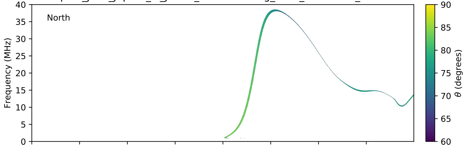
expres_juno_jupiter_io_jrm09_lossc-wid1deg_3kev_20170724_v01.cdf
