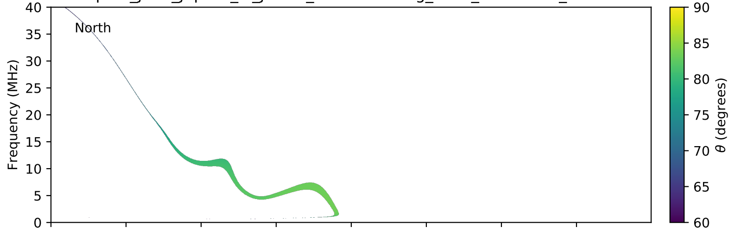
expres_juno_jupiter_io_jrm09_lossc-wid1deg_3kev_20170723_v01.cdf
