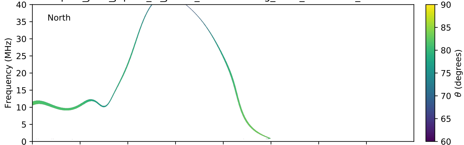
expres_juno_jupiter_io_jrm09_lossc-wid1deg_3kev_20170721_v01.cdf
