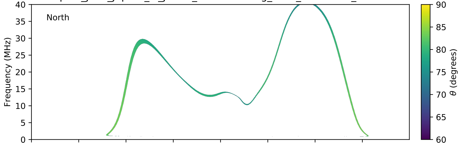
expres_juno_jupiter_io_jrm09_lossc-wid1deg_3kev_20170719_v01.cdf
