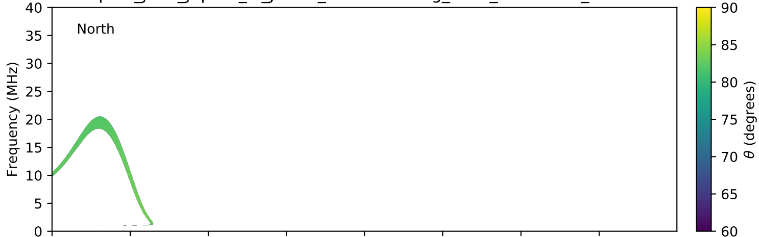
expres_juno_jupiter_io_jrm09_lossc-wid1deg_3kev_20170718_v01.cdf
