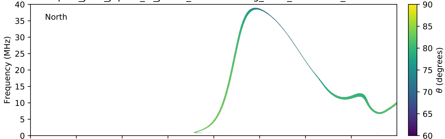
expres_juno_jupiter_io_jrm09_lossc-wid1deg_3kev_20170717_v01.cdf
