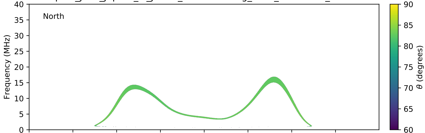
expres_juno_jupiter_io_jrm09_lossc-wid1deg_3kev_20170712_v01.cdf
