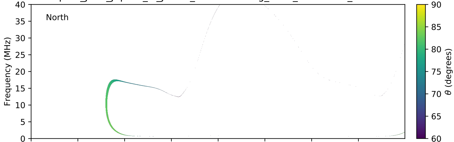
expres_juno_jupiter_io_jrm09_lossc-wid1deg_3kev_20170710_v01.cdf
