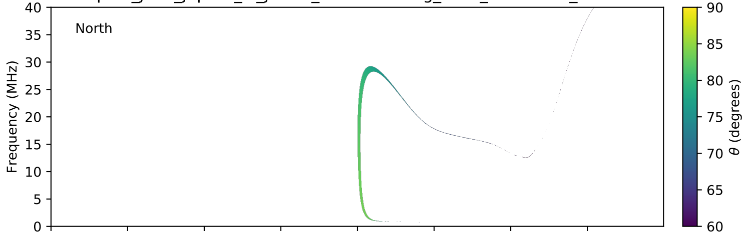
expres_juno_jupiter_io_jrm09_lossc-wid1deg_3kev_20170708_v01.cdf
