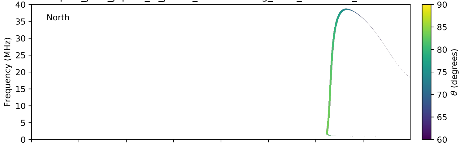
expres_juno_jupiter_io_jrm09_lossc-wid1deg_3kev_20170706_v01.cdf
