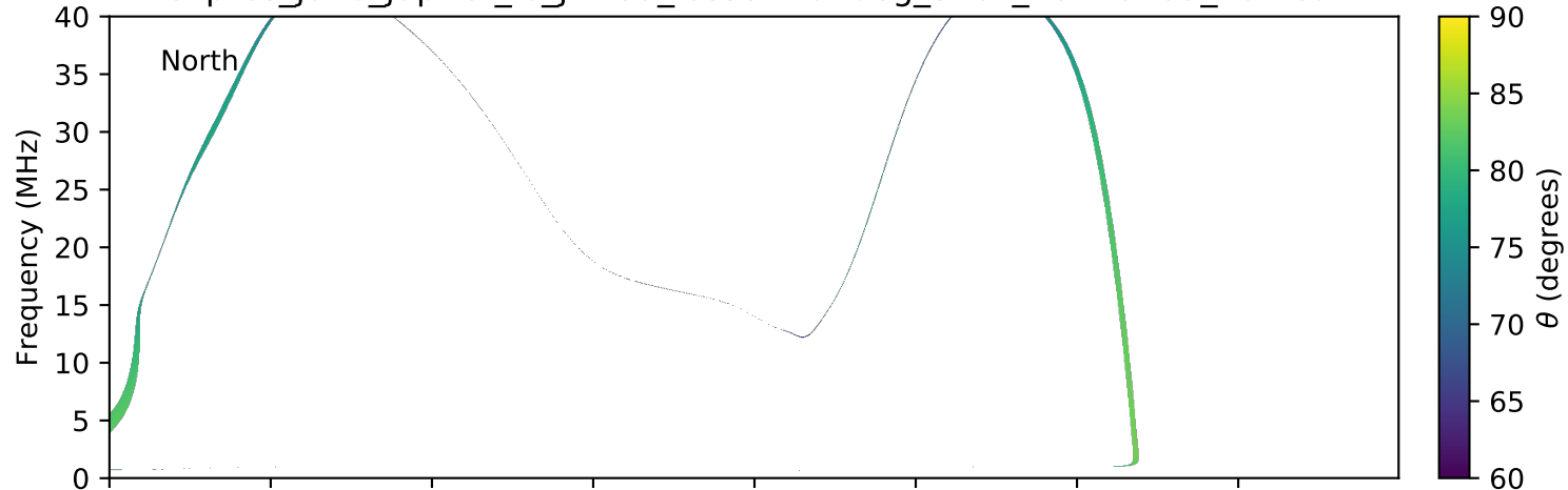
expres_juno_jupiter_io_jrm09_lossc-wid1deg_3kev_20170705_v01.cdf
