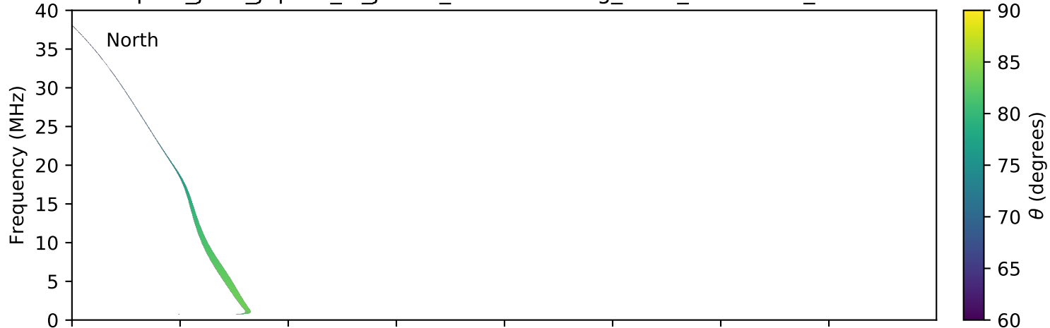
expres_juno_jupiter_io_jrm09_lossc-wid1deg_3kev_20170702_v01.cdf
